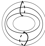
Figure 2. Two lightcones in \mathrm{Ein}^{1,1} .
