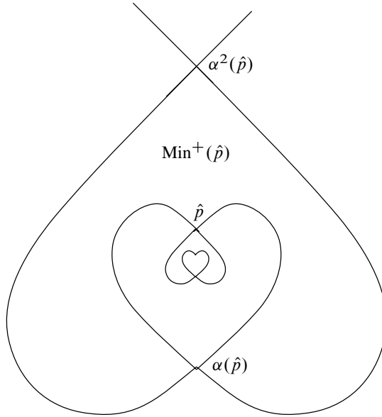
Figure 3. A Minkowski patch in \widetilde{\text{Ein}}^{1,1} .
